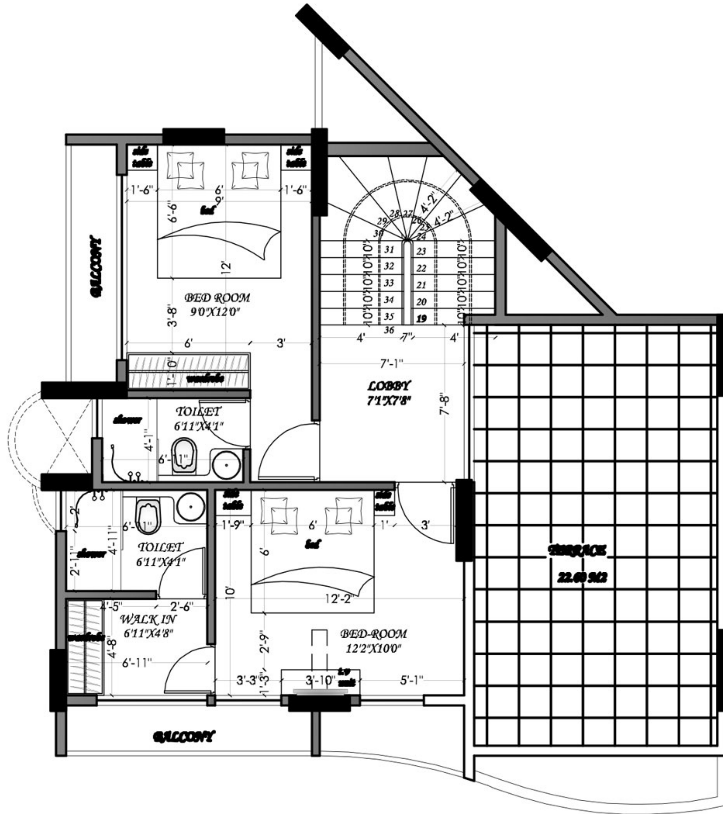
14TH FLOOR PLAN
